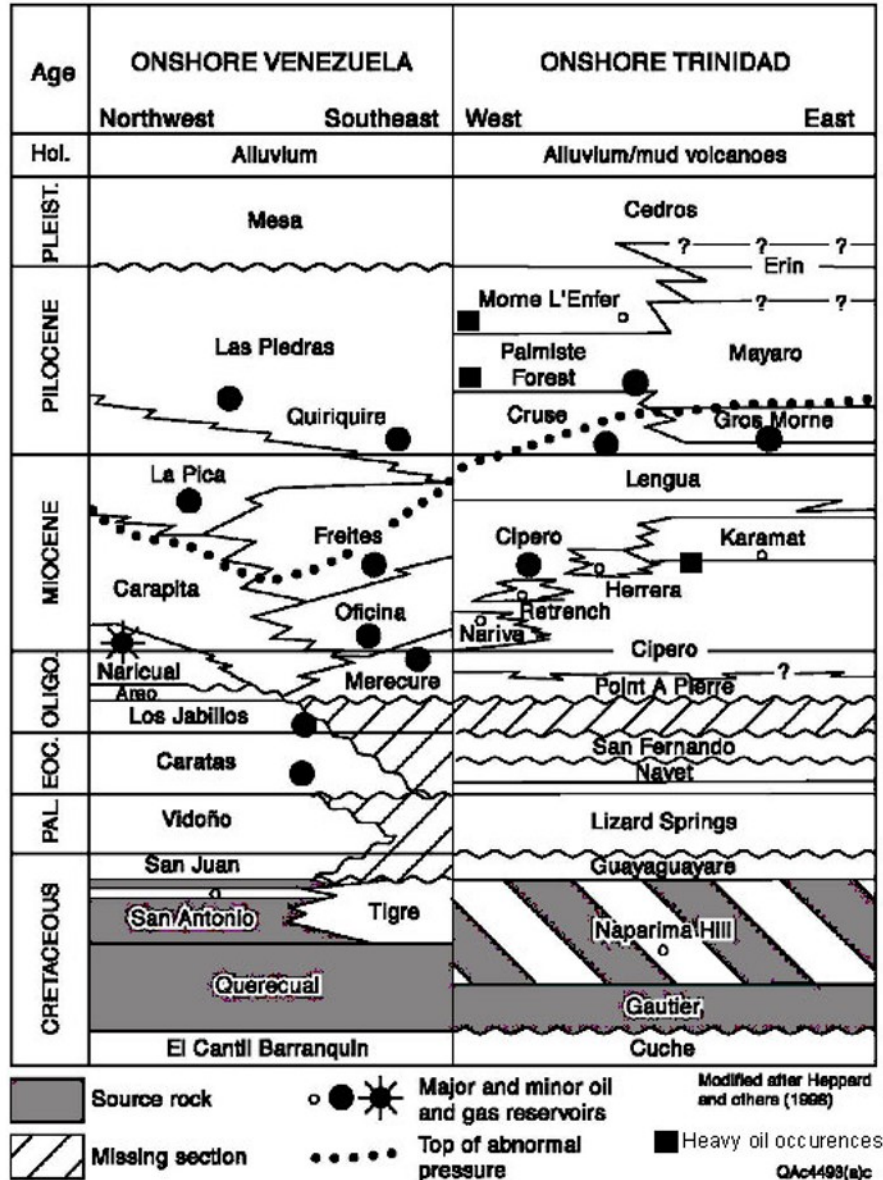
Generalized stratigraphic column of Eastern Venezuela-Trinidad stratigraphy with heavy oil-oil sand occurrences marked with solid squares (modified from Heppard et al., 1998).
